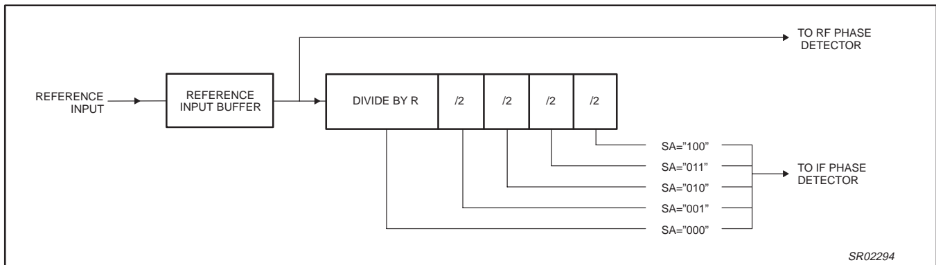
Figure 5. Reference divider.
